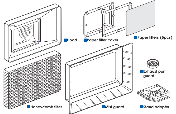
FT-03S HOOD SET FOR Mr.SUPER COMPACT BOOTH
